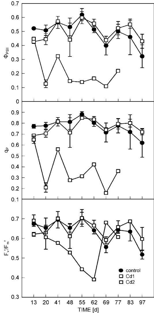
Fig. 5. Parameters of chlorophyll fluorescence ( \Phi_{PSII} , q_P , F_v'/F_m' ) during the 97-d trail ( n = 3 - 6 , n = 1 for Cd2 plants after day 20).
