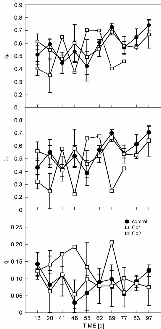
Fig. 7. Fluorescence quenching ( q_N , q_F and q_I values) during the 97-d trail ( n = 3 - 6 , n = 1 for Cd2 plants after day 20).
