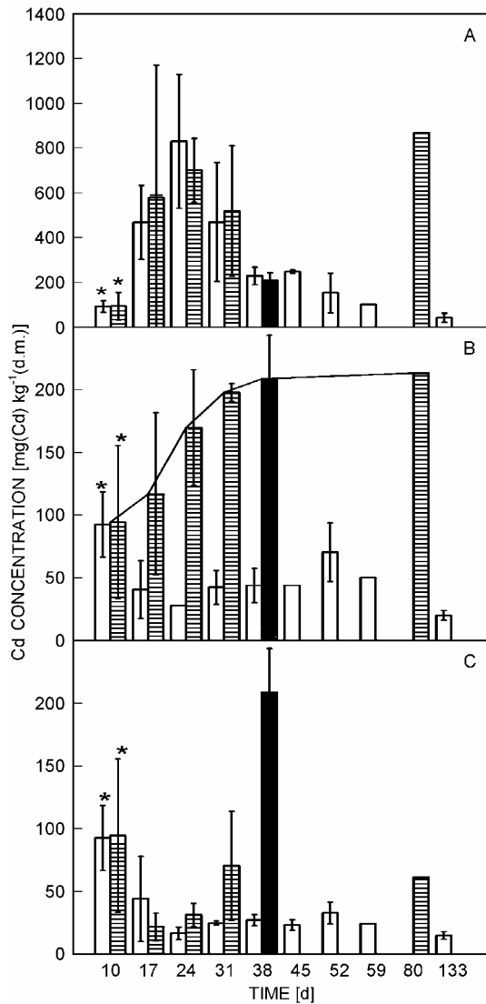
Fig. 2. Cd accumulation in roots (A), stems (B) and leaves (C) of hemp plants grown on cadmium contaminated soil. Cd determination 10 d after sowing was carried out with the whole plant, separation in different plant parts was not possible. The Cd concentration of the Cd2 plant 38 d after sowing was markedly different because it primarily represents the stem (open columns - Cd1, striped columns - Cd2, closed columns - primarily stem, * - whole plants) ( n = 2 - 6 , n = 1 for Cd2 plant 80 d after sowing).
