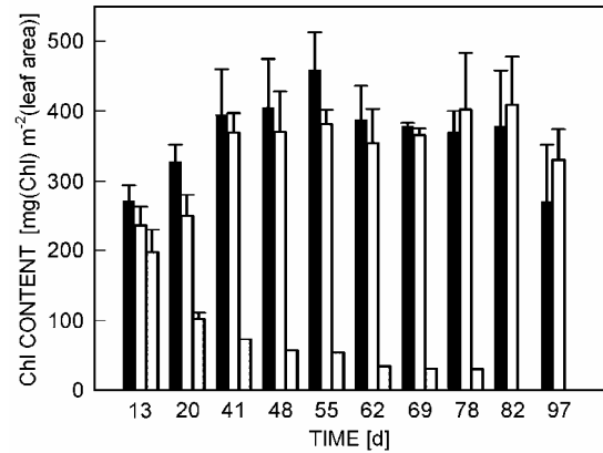
Fig. 3. Chlorophyll content during the 97-d trail (closed columns - control, open columns - Cd1, grey columns - Cd2) ( n = 3 - 6 , n = 1 for Cd2 plants after day 20).
